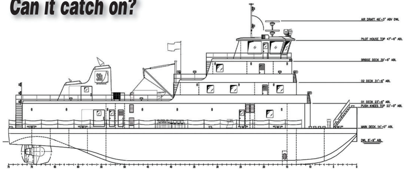
OUTBOARD PROFILE
